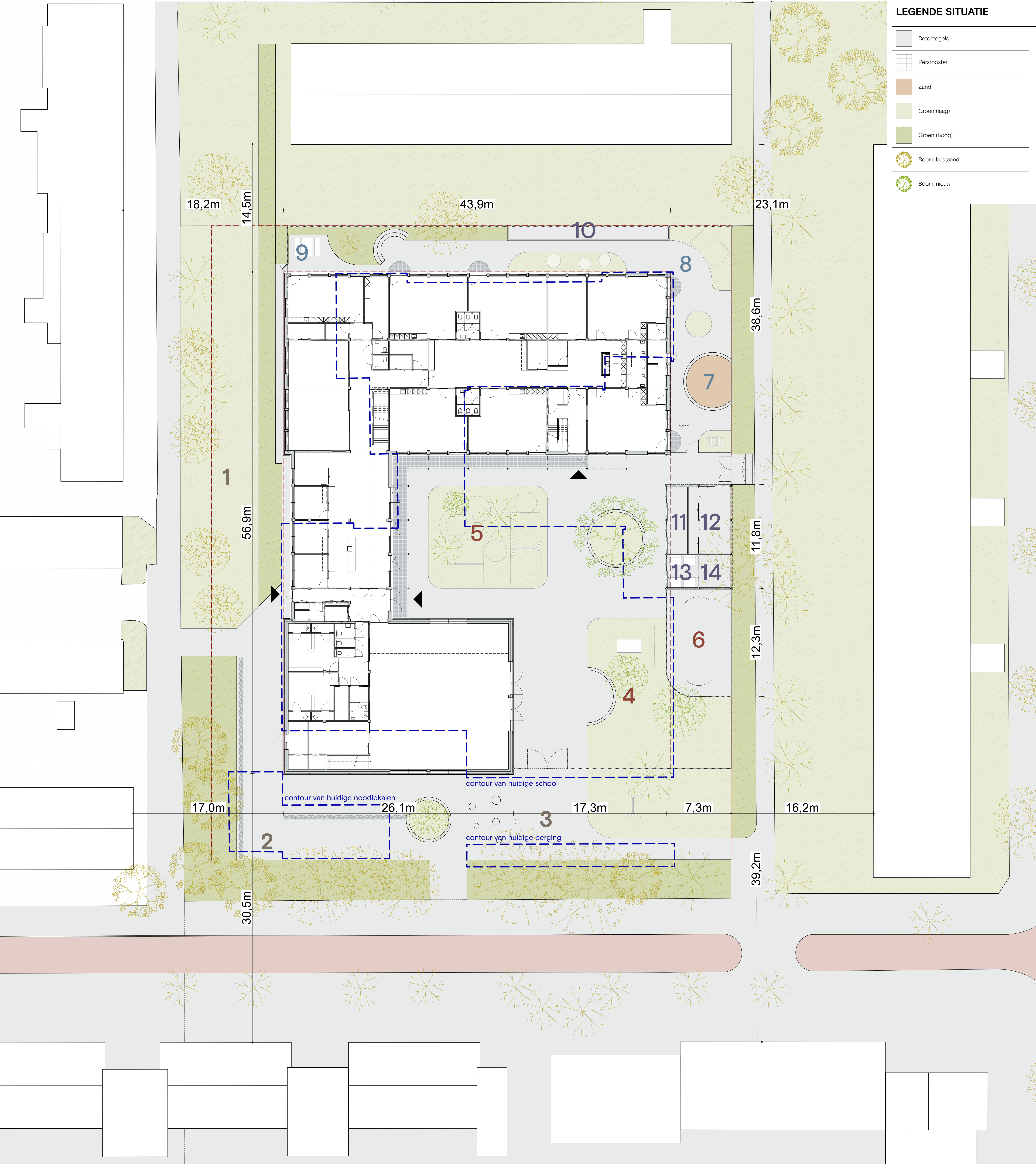
Inplantingsplan. 1:150
